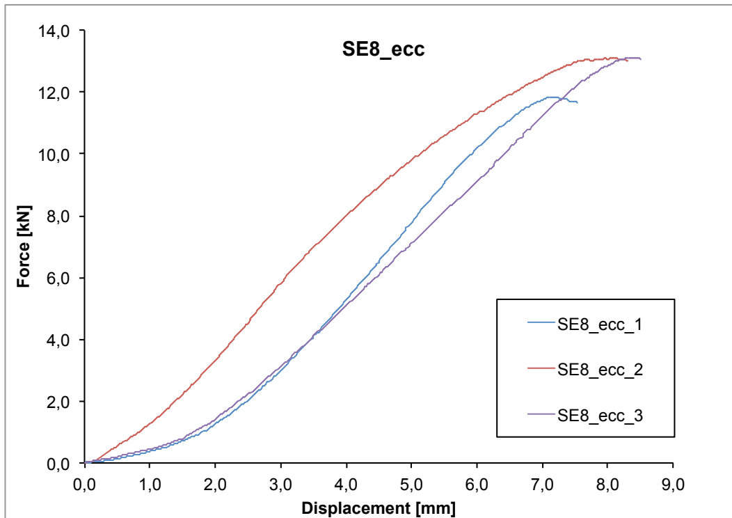
Figure 1 Diagram force versus displacement of testing machine's crossbar for "ETERNO SE8" specimen.
