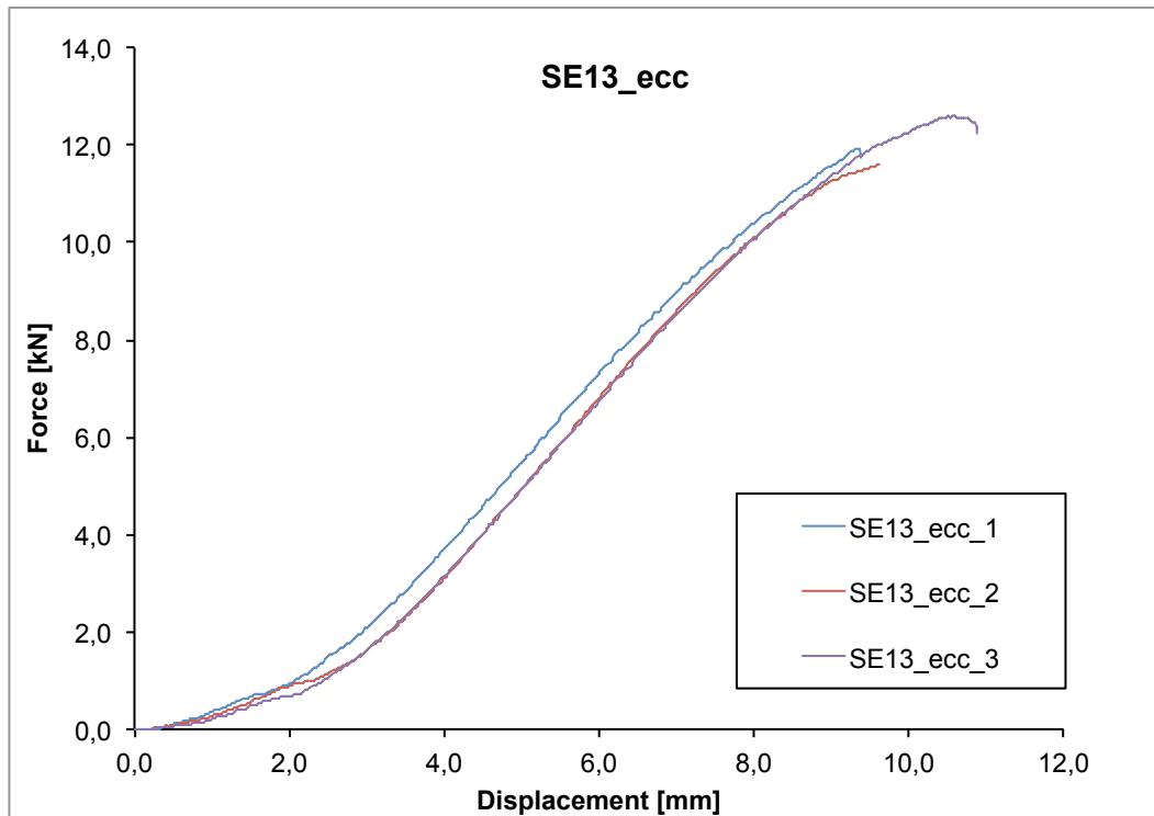
Figure 1 Diagram force versus displacement of testing machine's crossbar for "ETERNO SE13" specimen.
