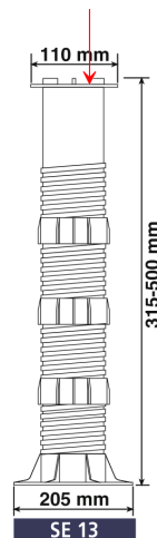
Figure 2 Typical "ETERNO SE13" specimen.
